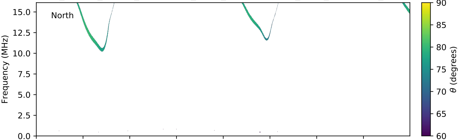
expres_cassini_jupiter_ganymede_isaac_lossc-wid1deg_3kev_20021227_v01.cdf
