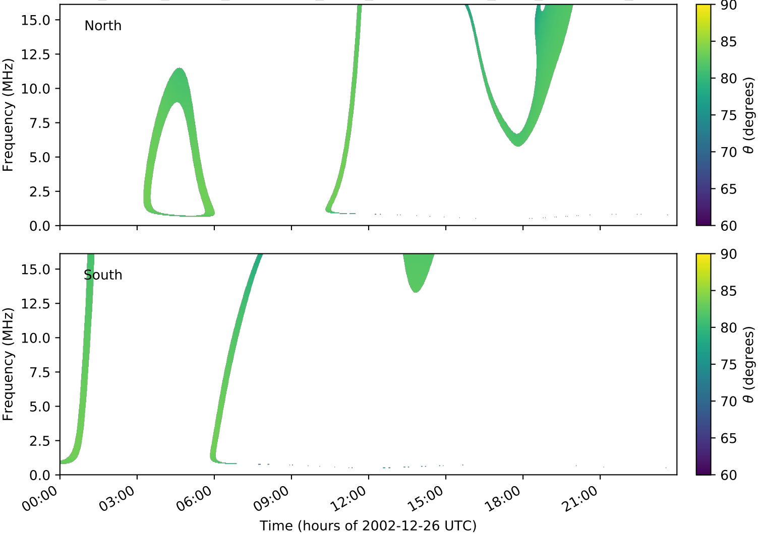
expres_cassini_jupiter_ganymede_isaac_lossc-wid1deg_3kev_20021226_v01.cdf
