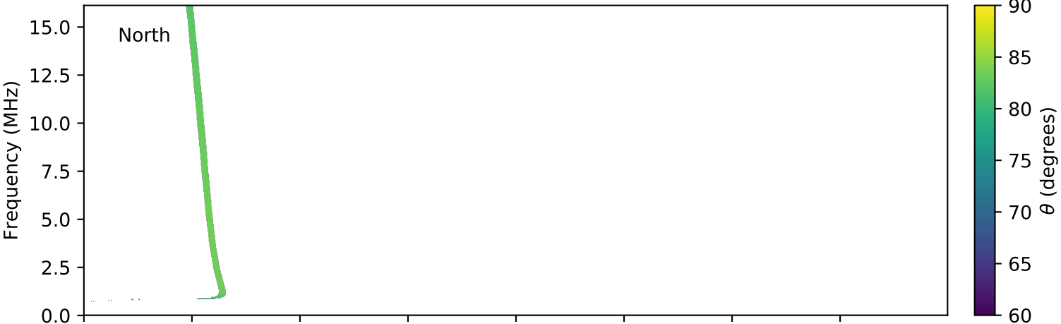
expres_cassini_jupiter_ganymede_isaac_lossc-wid1deg_3kev_20021222_v01.cdf
