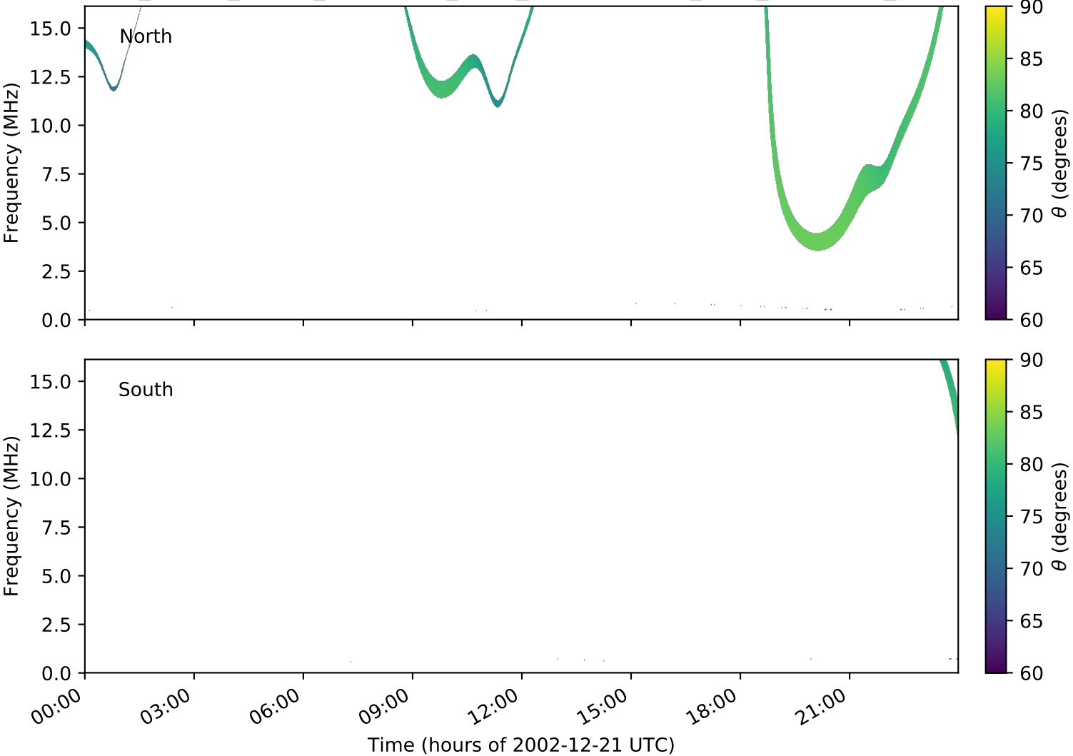
expres_cassini_jupiter_ganymede_isaac_lossc-wid1deg_3kev_20021221_v01.cdf
