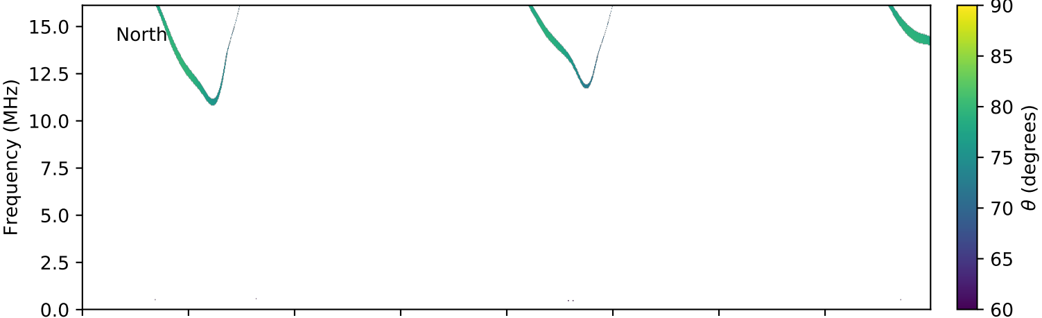
expres_cassini_jupiter_ganymede_isaac_lossc-wid1deg_3kev_20021220_v01.cdf
