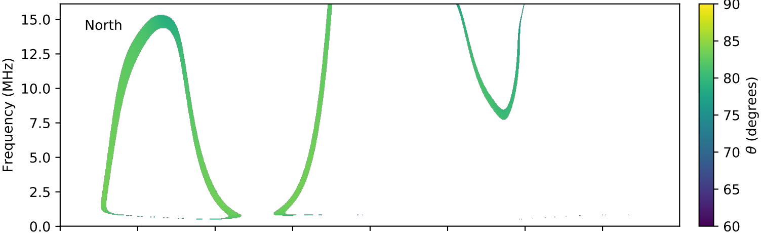
expres_cassini_jupiter_ganymede_isaac_lossc-wid1deg_3kev_20021219_v01.cdf
