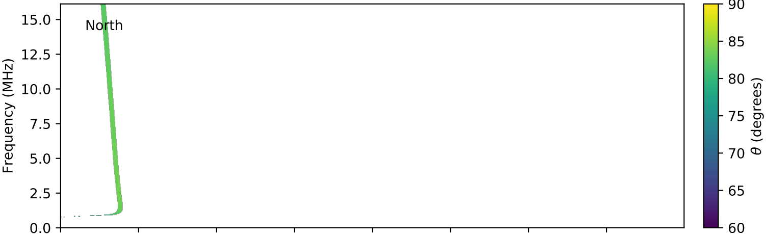
expres_cassini_jupiter_ganymede_isaac_lossc-wid1deg_3kev_20021215_v01.cdf
