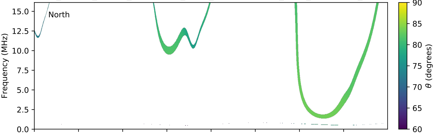
expres_cassini_jupiter_ganymede_isaac_lossc-wid1deg_3kev_20021214_v01.cdf
