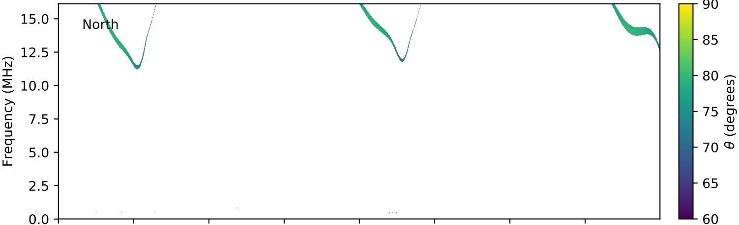
expres_cassini_jupiter_ganymede_isaac_lossc-wid1deg_3kev_20021213_v01.cdf
