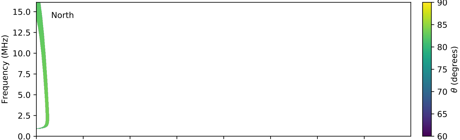
expres_cassini_jupiter_ganymede_isaac_lossc-wid1deg_3kev_20021208_v01.cdf
