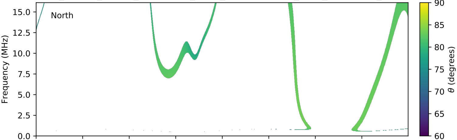
expres_cassini_jupiter_ganymede_isaac_lossc-wid1deg_3kev_20021207_v01.cdf
