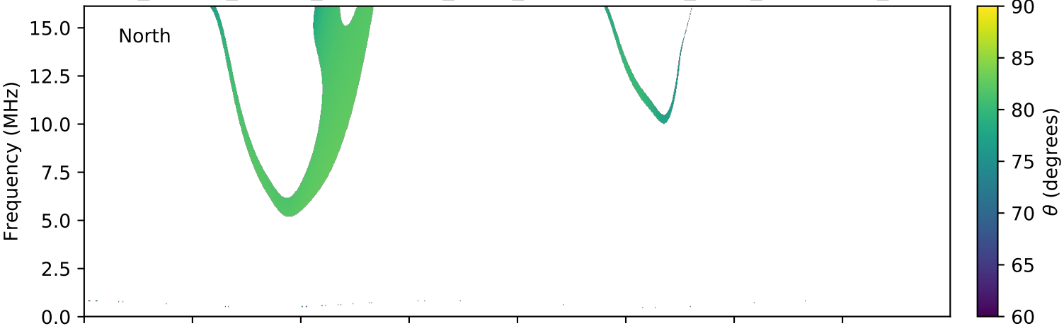
expres_cassini_jupiter_ganymede_isaac_lossc-wid1deg_3kev_20021205_v01.cdf
