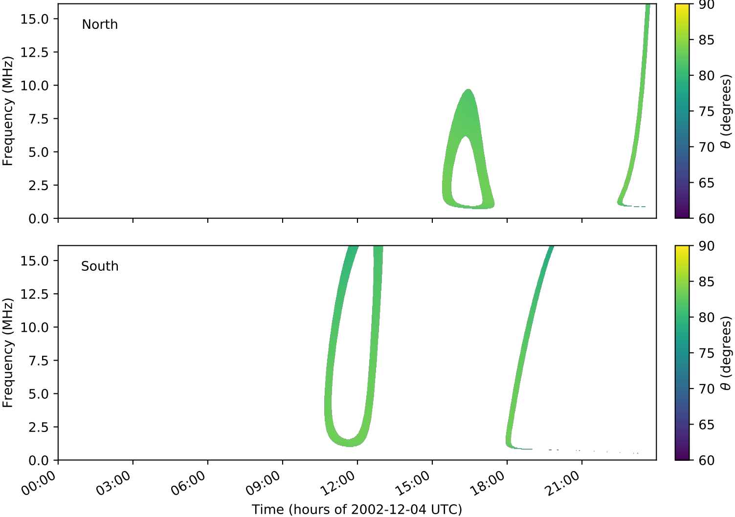
expres_cassini_jupiter_ganymede_isaac_lossc-wid1deg_3kev_20021204_v01.cdf
