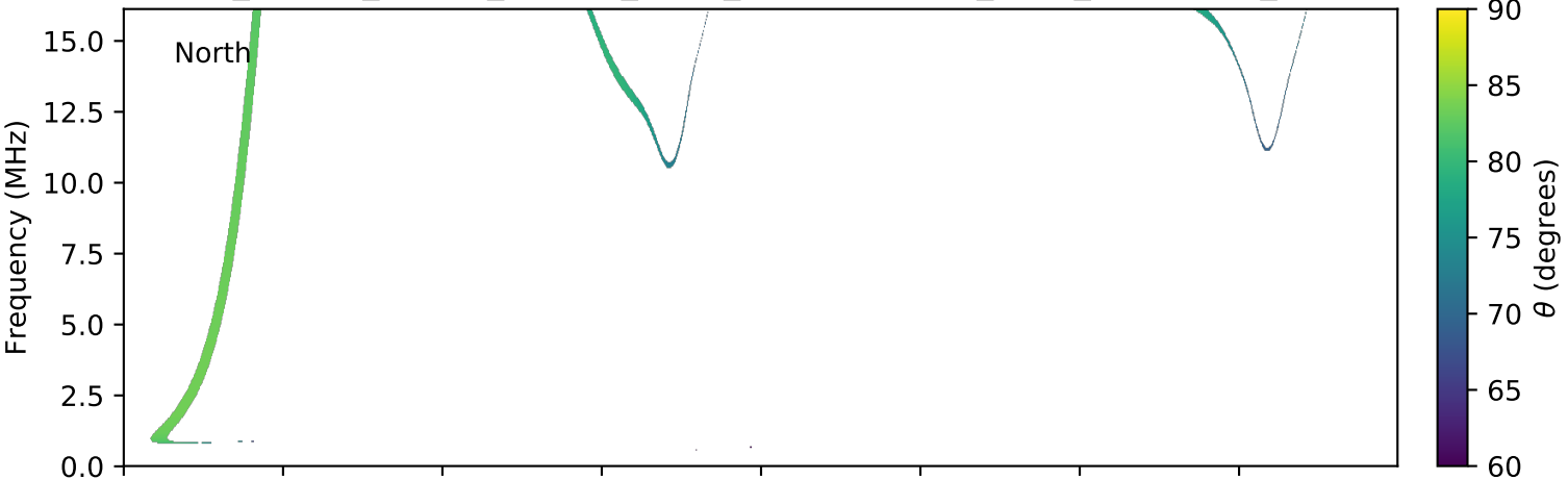
expres_cassini_jupiter_europa_isaac_lossc-wid1deg_3kev_20021228_v01.cdf
