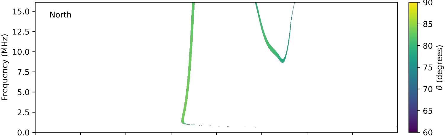
expres_cassini_jupiter_europa_isaac_lossc-wid1deg_3kev_20021224_v01.cdf
