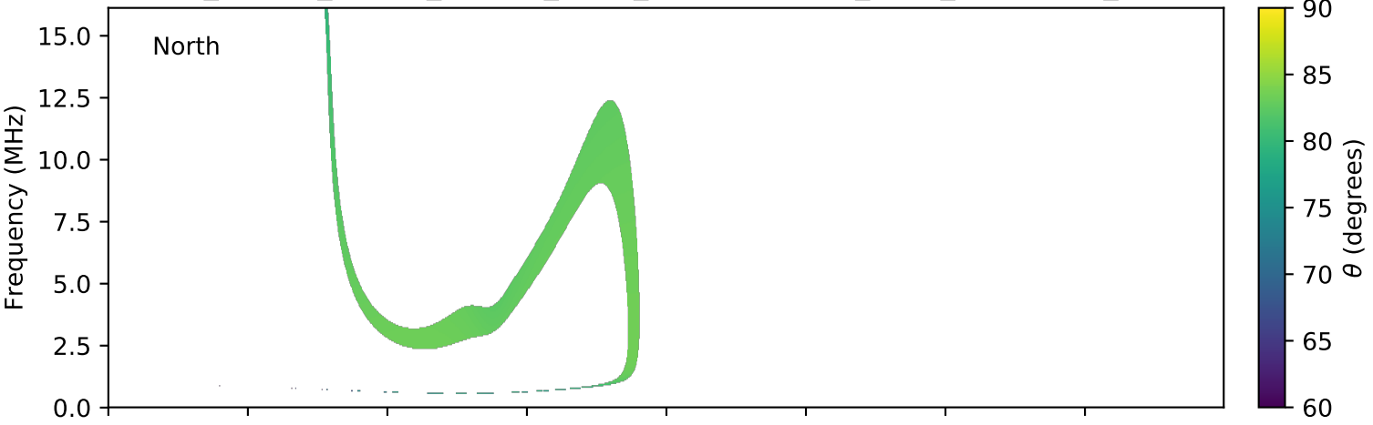
expres_cassini_jupiter_europa_isaac_lossc-wid1deg_3kev_20021222_v01.cdf
