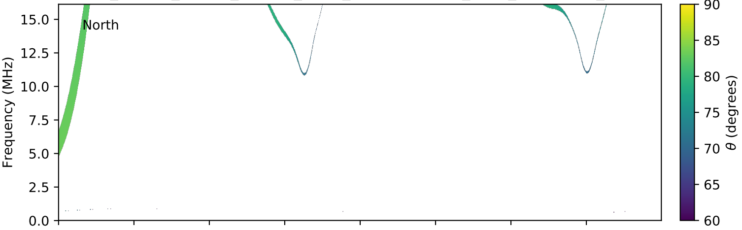
expres_cassini_jupiter_europa_isaac_lossc-wid1deg_3kev_20021221_v01.cdf
