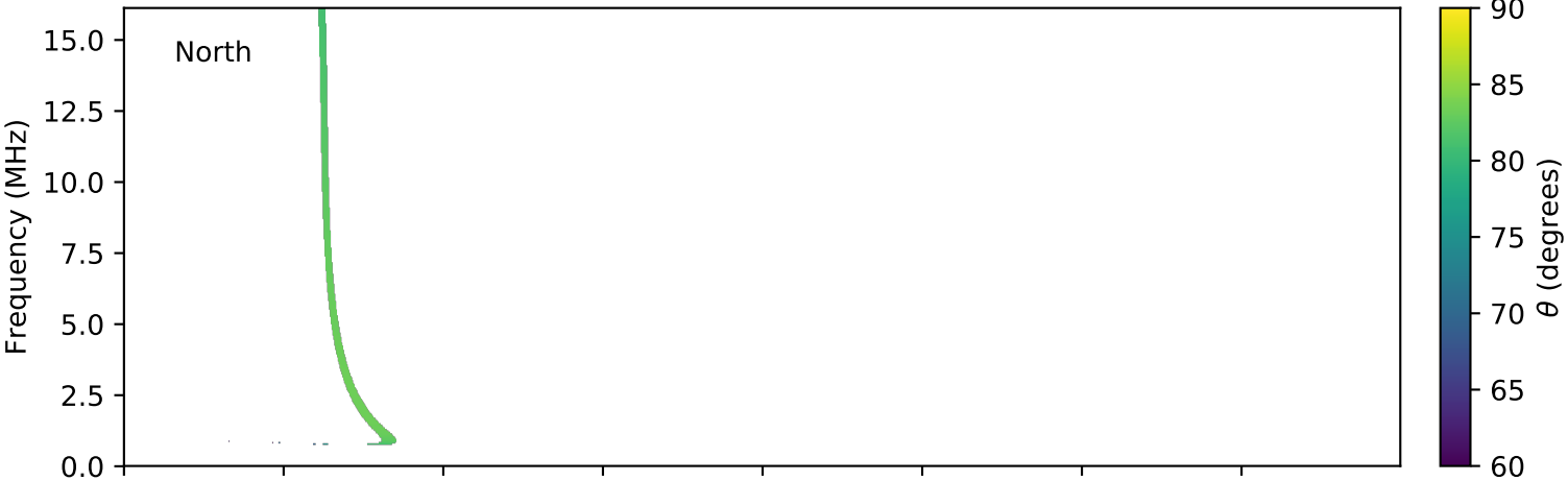
expres_cassini_jupiter_europa_isaac_lossc-wid1deg_3kev_20021215_v01.cdf
