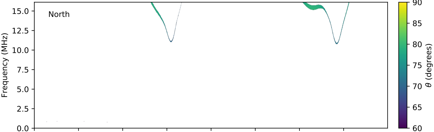
expres_cassini_jupiter_europa_isaac_lossc-wid1deg_3kev_20021214_v01.cdf
