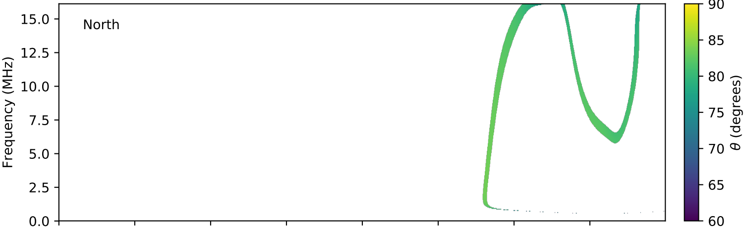
expres_cassini_jupiter_europa_isaac_lossc-wid1deg_3kev_20021213_v01.cdf
