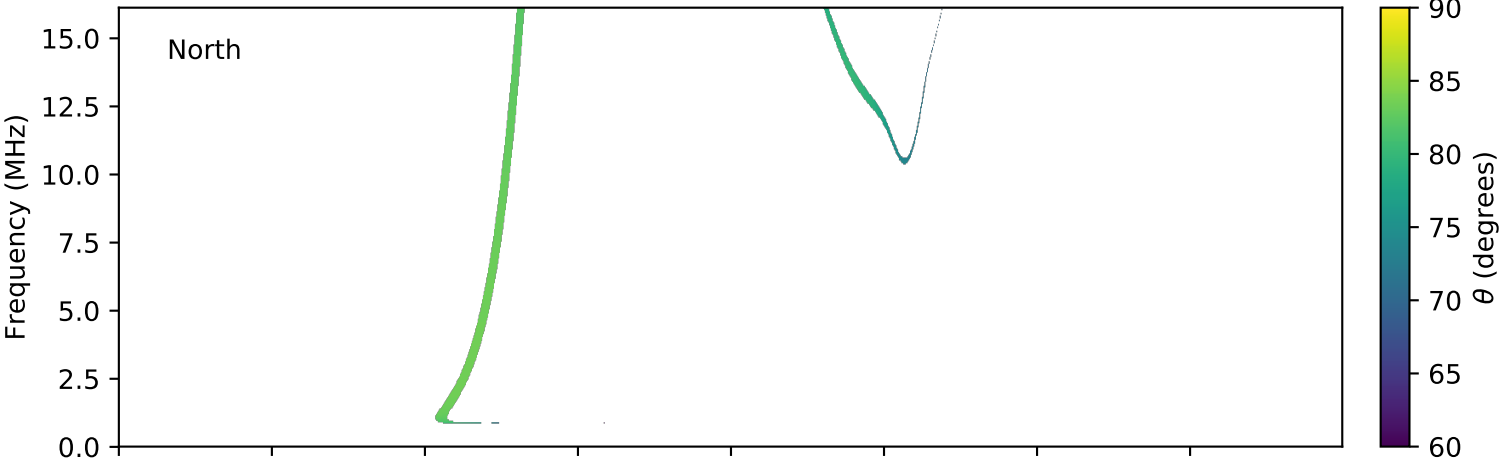
expres_cassini_jupiter_europa_isaac_lossc-wid1deg_3kev_20021210_v01.cdf
