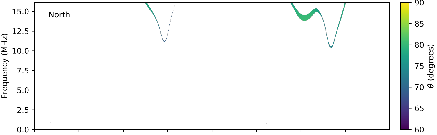
expres_cassini_jupiter_europa_isaac_lossc-wid1deg_3kev_20021207_v01.cdf
