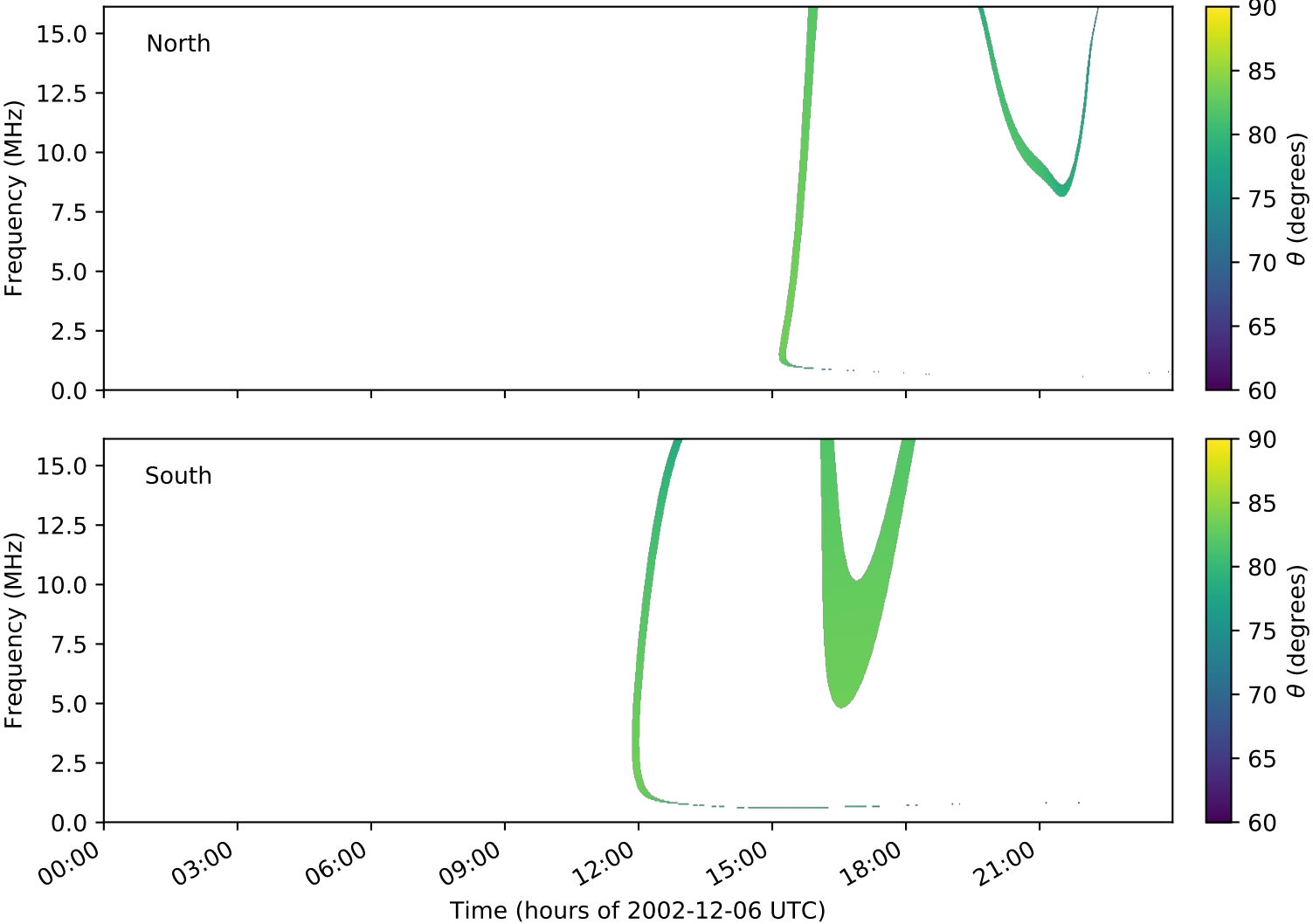
expres_cassini_jupiter_europa_isaac_lossc-wid1deg_3kev_20021206_v01.cdf
