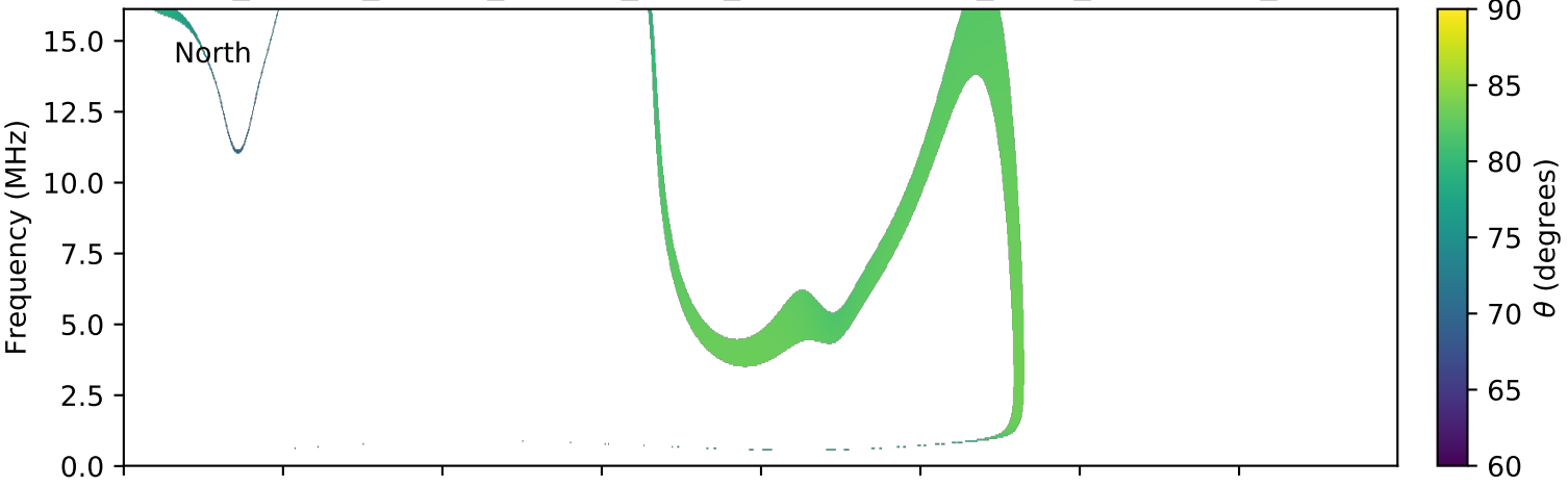
expres_cassini_jupiter_europa_isaac_lossc-wid1deg_3kev_20021204_v01.cdf
