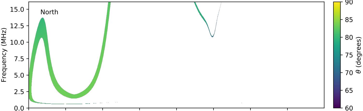
expres_cassini_jupiter_europa_isaac_lossc-wid1deg_3kev_20021203_v01.cdf
