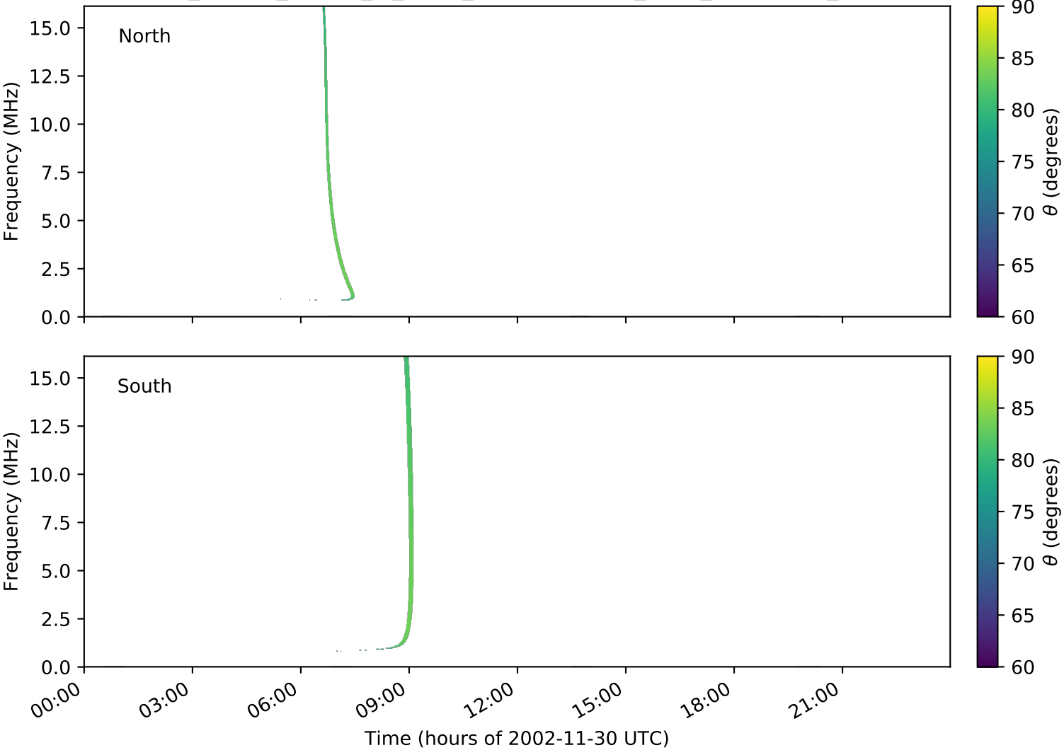
expres_cassini_jupiter_io_isaac_lossc-wid1deg_3kev_20021130_v01.cdf
