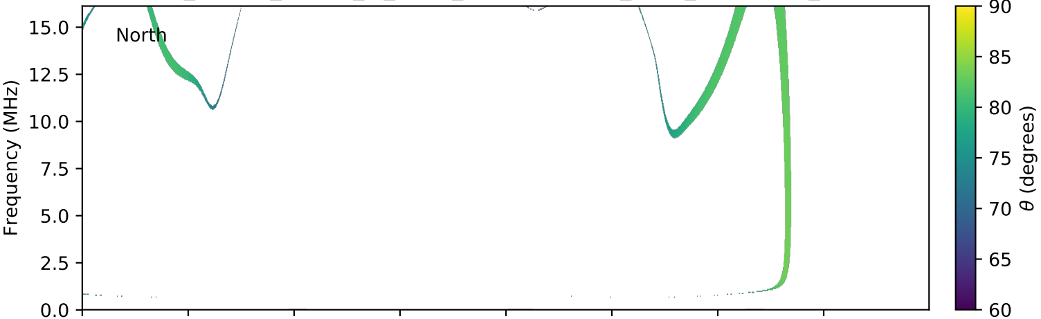
expres_cassini_jupiter_io_isaac_lossc-wid1deg_3kev_20021126_v01.cdf
