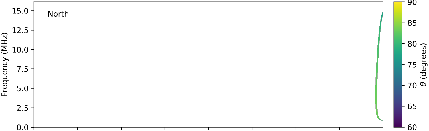
expres_cassini_jupiter_io_isaac_lossc-wid1deg_3kev_20021125_v01.cdf
