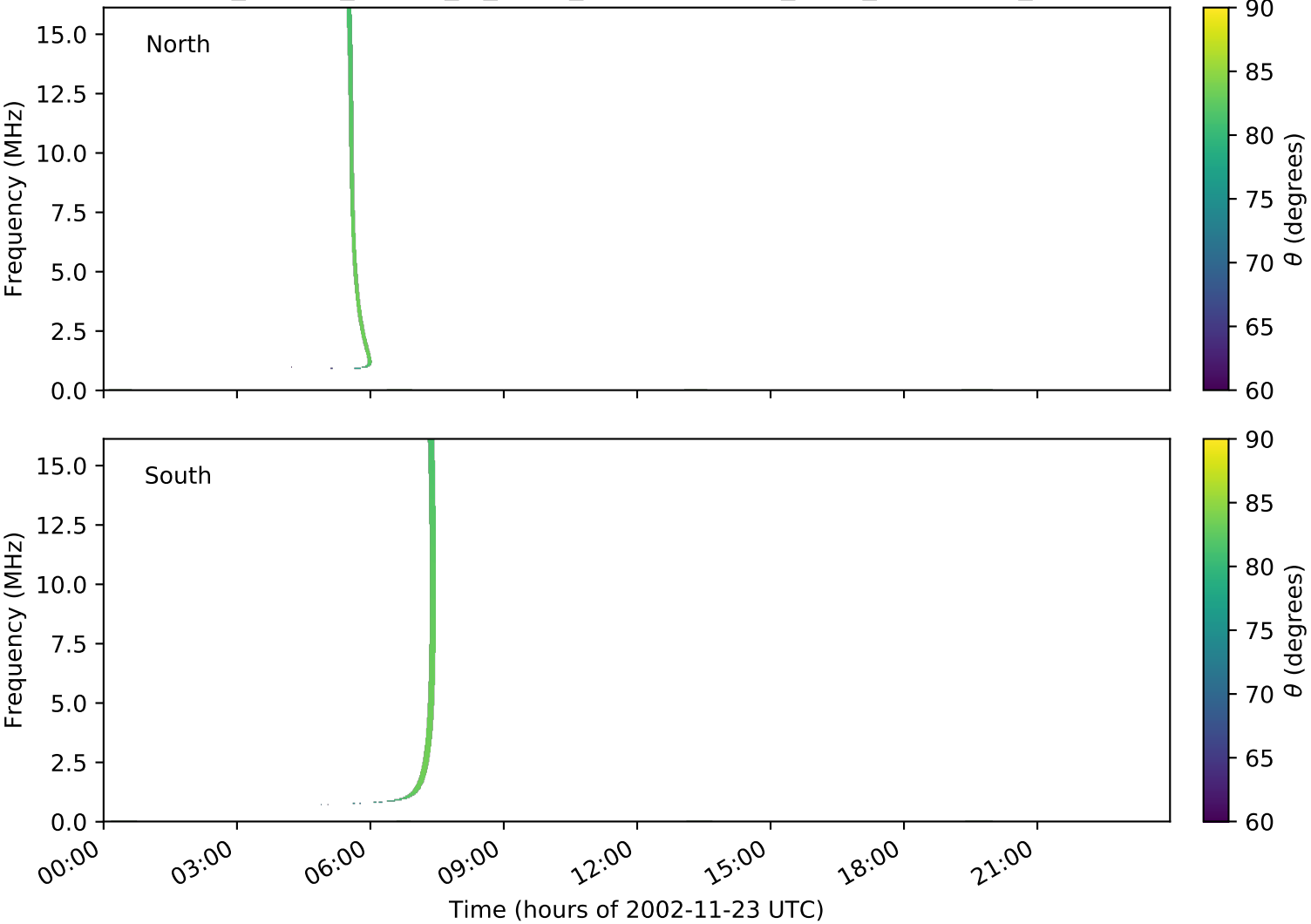
expres_cassini_jupiter_io_isaac_lossc-wid1deg_3kev_20021123_v01.cdf
