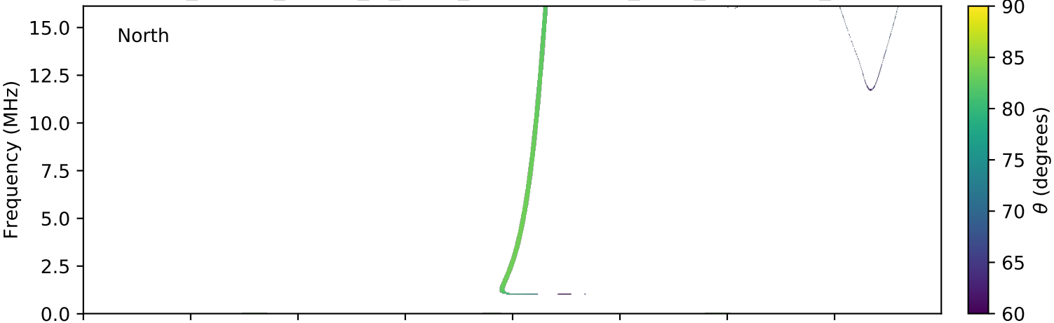
expres_cassini_jupiter_io_isaac_lossc-wid1deg_3kev_20021122_v01.cdf
