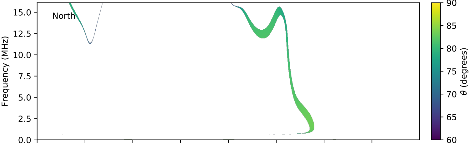
expres_cassini_jupiter_io_isaac_lossc-wid1deg_3kev_20021119_v01.cdf
