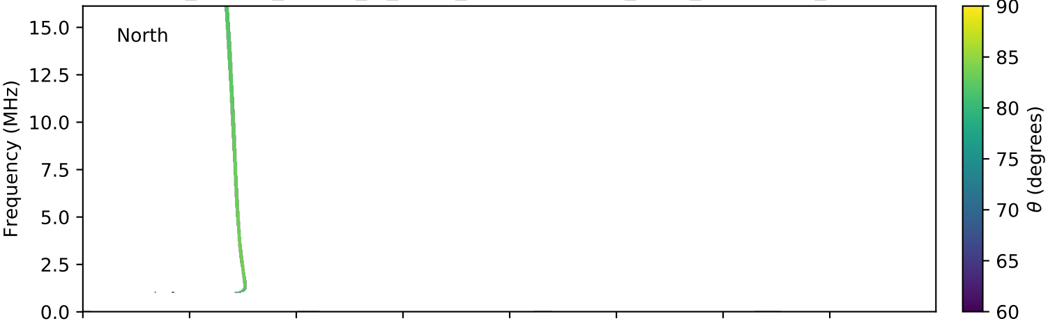
expres_cassini_jupiter_io_isaac_lossc-wid1deg_3kev_20021116_v01.cdf
