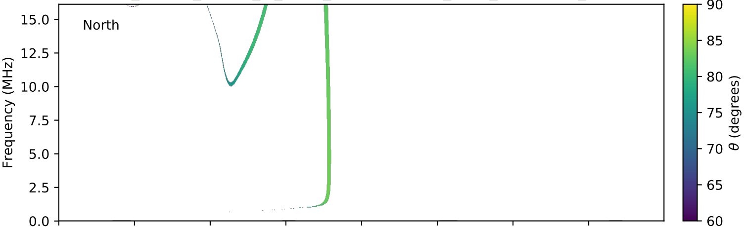
expres_cassini_jupiter_io_isaac_lossc-wid1deg_3kev_20021114_v01.cdf
