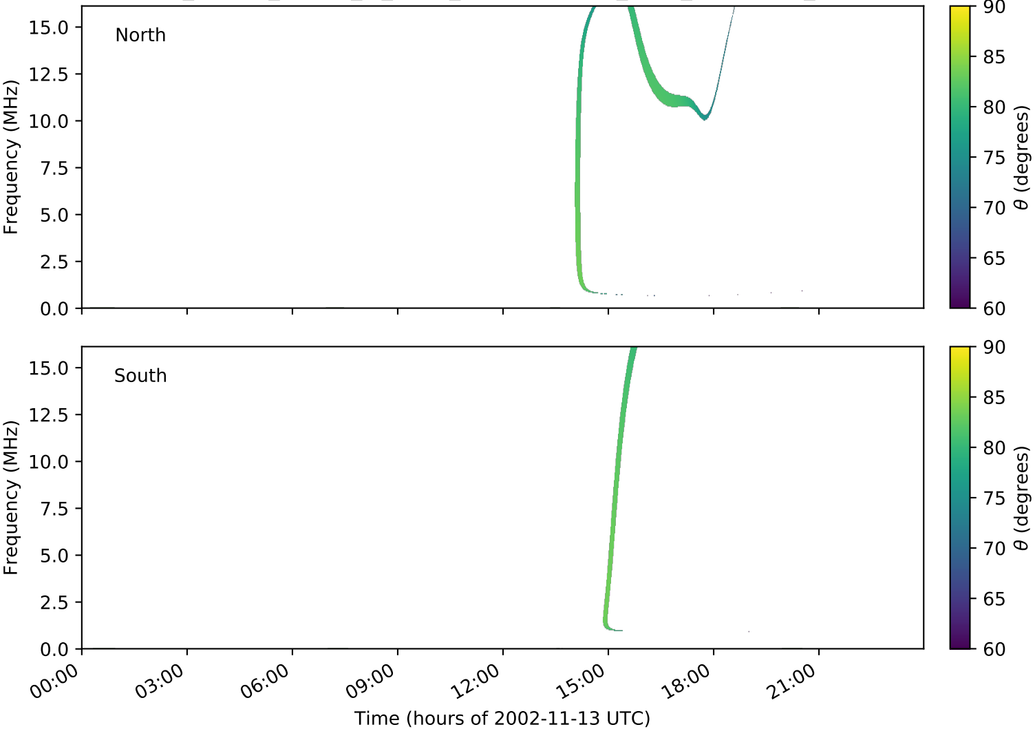
expres_cassini_jupiter_io_isaac_lossc-wid1deg_3kev_20021113_v01.cdf
