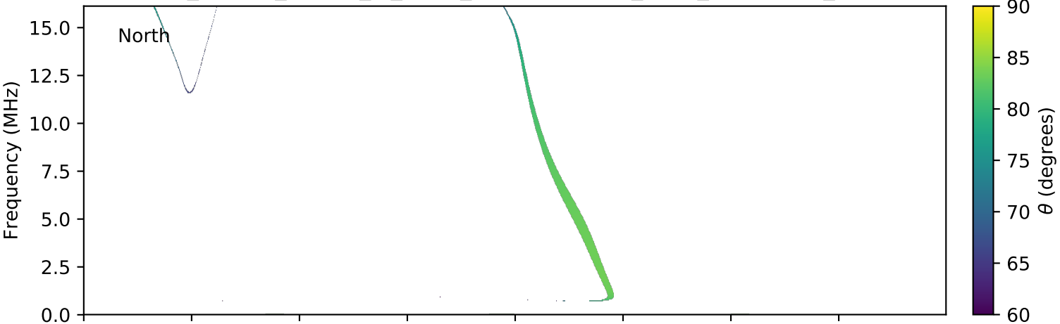
expres_cassini_jupiter_io_isaac_lossc-wid1deg_3kev_20021112_v01.cdf
