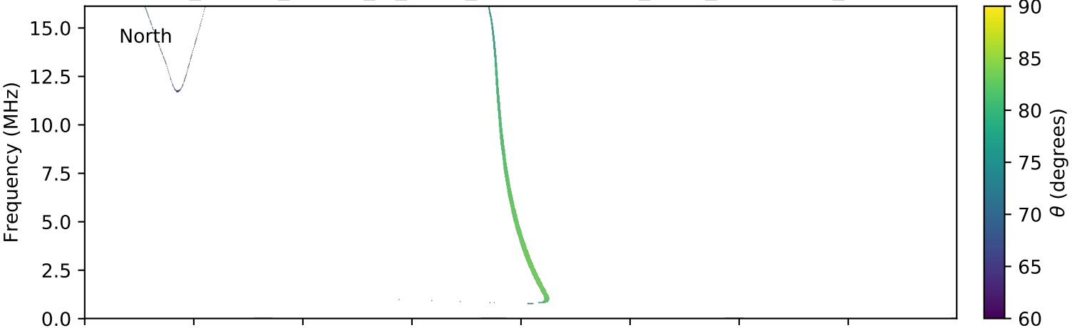
expres_cassini_jupiter_io_isaac_lossc-wid1deg_3kev_20021105_v01.cdf
