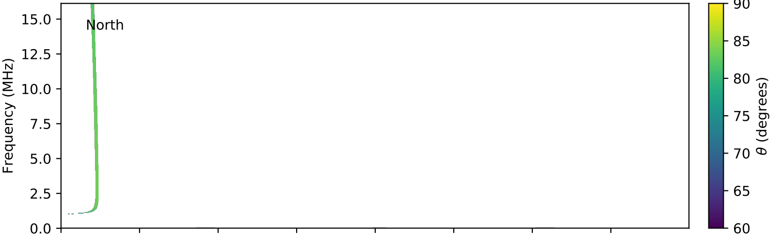
expres_cassini_jupiter_io_isaac_lossc-wid1deg_3kev_20021102_v01.cdf
