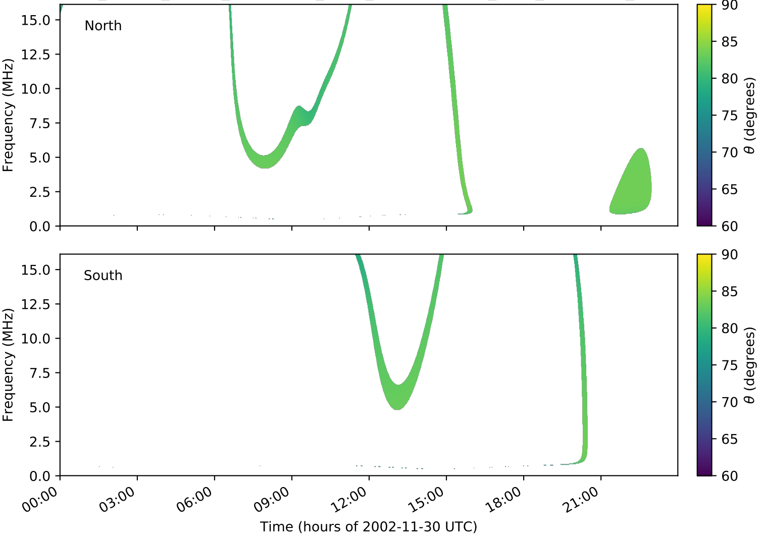
expres_cassini_jupiter_ganymede_isaac_lossc-wid1deg_3kev_20021130_v01.cdf
