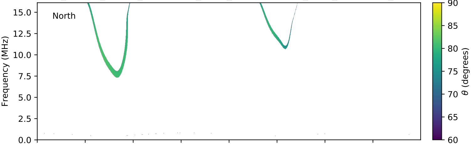
expres_cassini_jupiter_ganymede_isaac_lossc-wid1deg_3kev_20021128_v01.cdf
