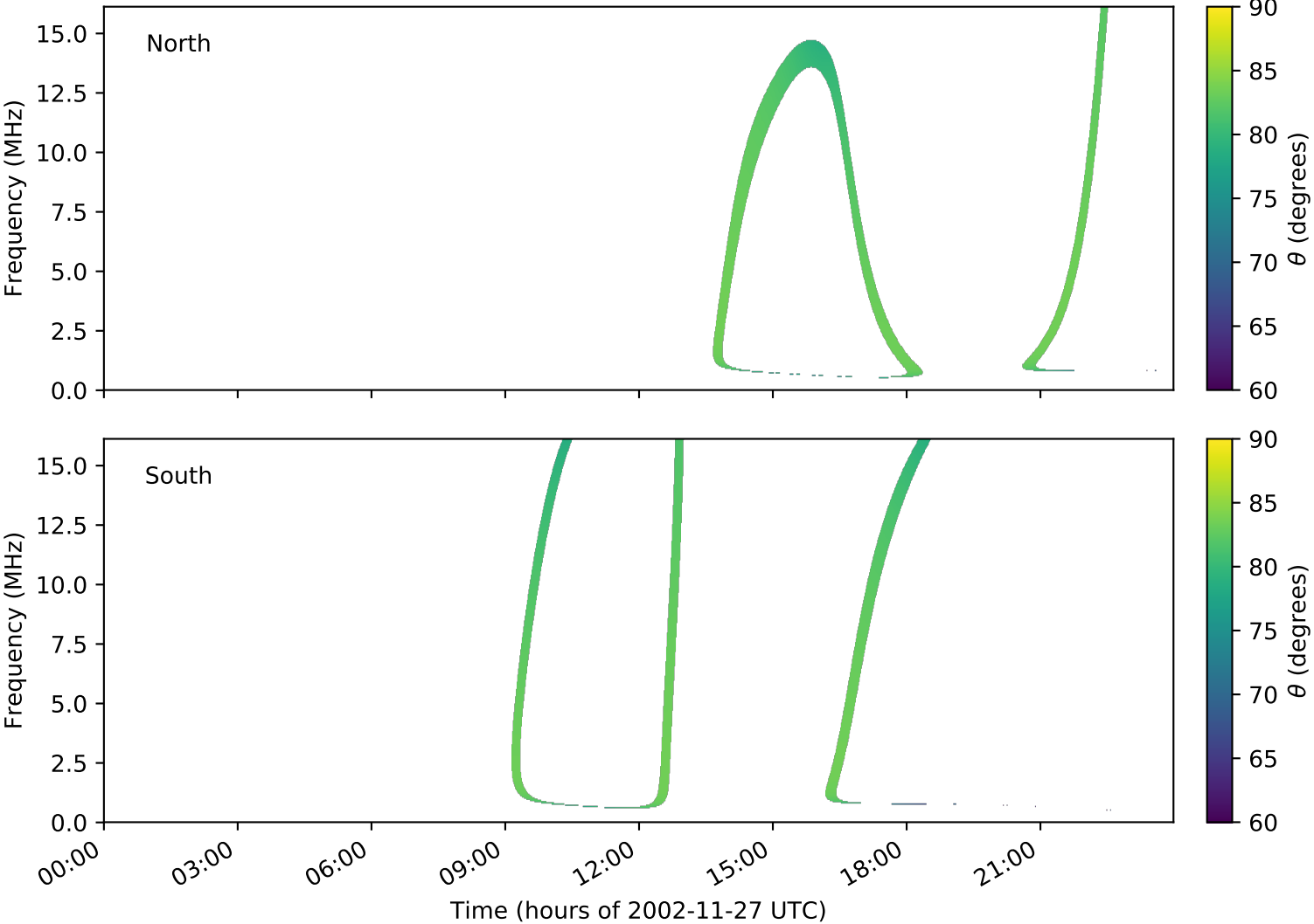
expres_cassini_jupiter_ganymede_isaac_lossc-wid1deg_3kev_20021127_v01.cdf
