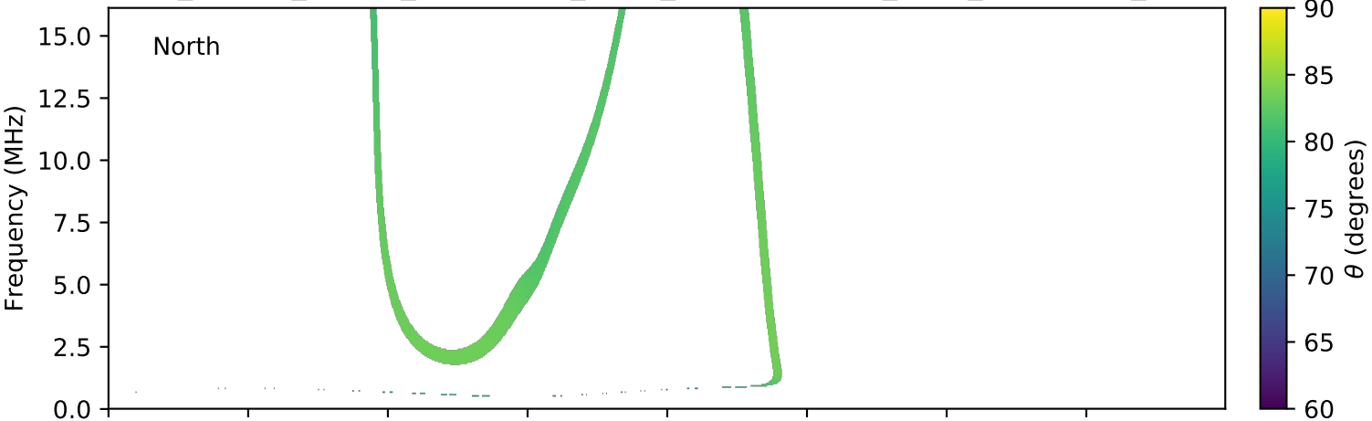
expres_cassini_jupiter_ganymede_isaac_lossc-wid1deg_3kev_20021123_v01.cdf
