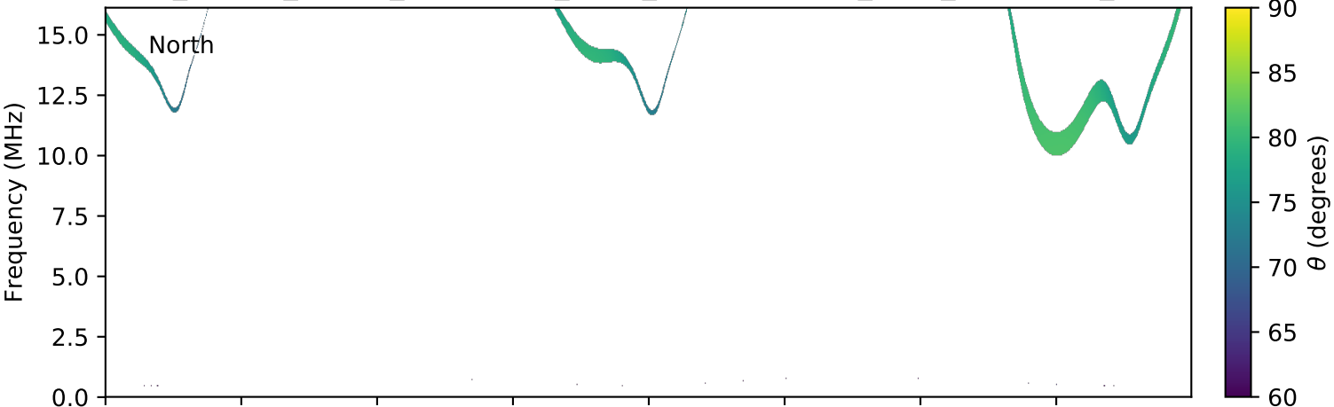
expres_cassini_jupiter_ganymede_isaac_lossc-wid1deg_3kev_20021122_v01.cdf
