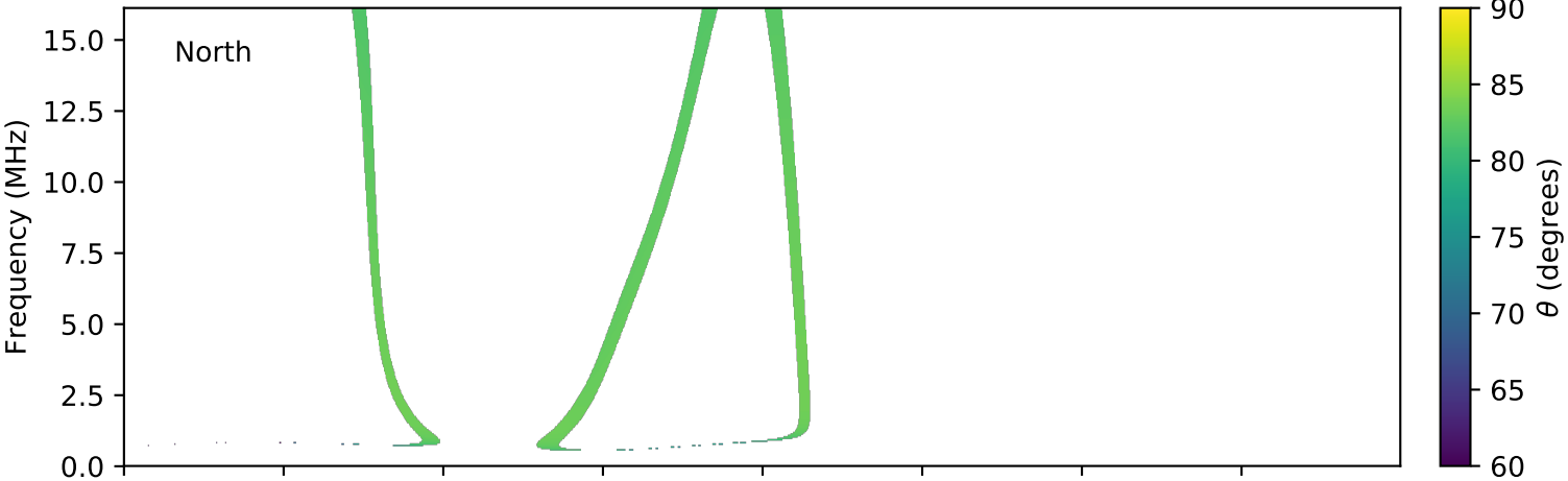
expres_cassini_jupiter_ganymede_isaac_lossc-wid1deg_3kev_20021116_v01.cdf
