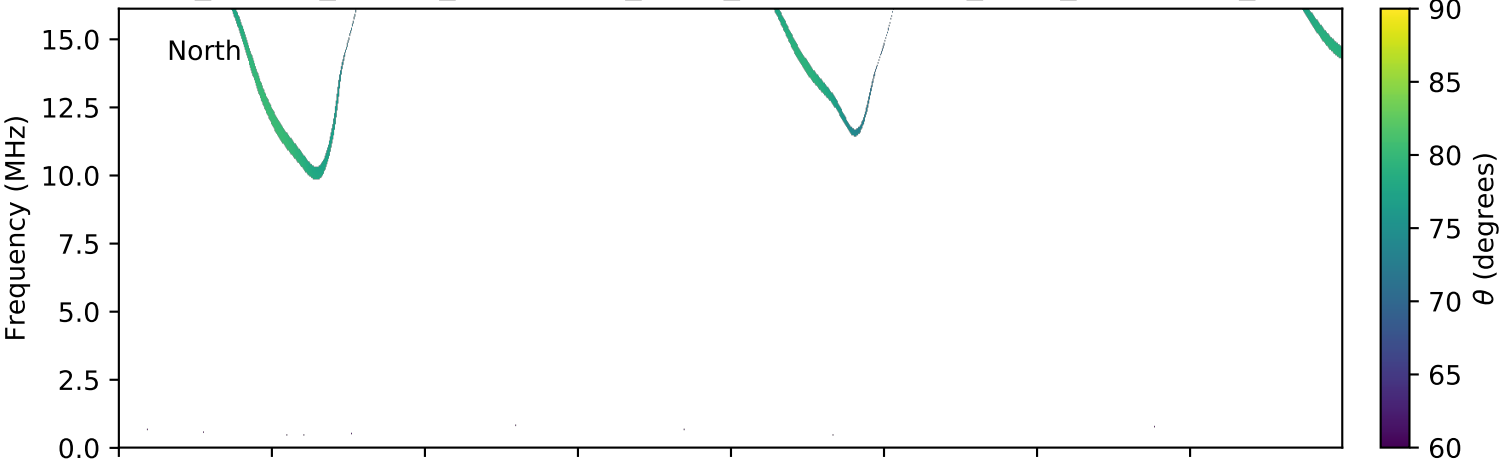
expres_cassini_jupiter_ganymede_isaac_lossc-wid1deg_3kev_20021114_v01.cdf
