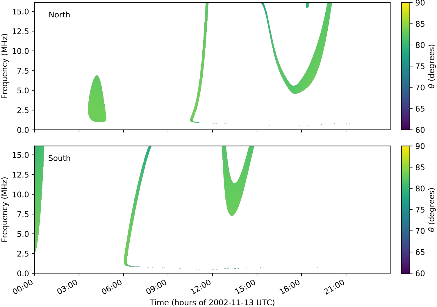
expres_cassini_jupiter_ganymede_isaac_lossc-wid1deg_3kev_20021113_v01.cdf
