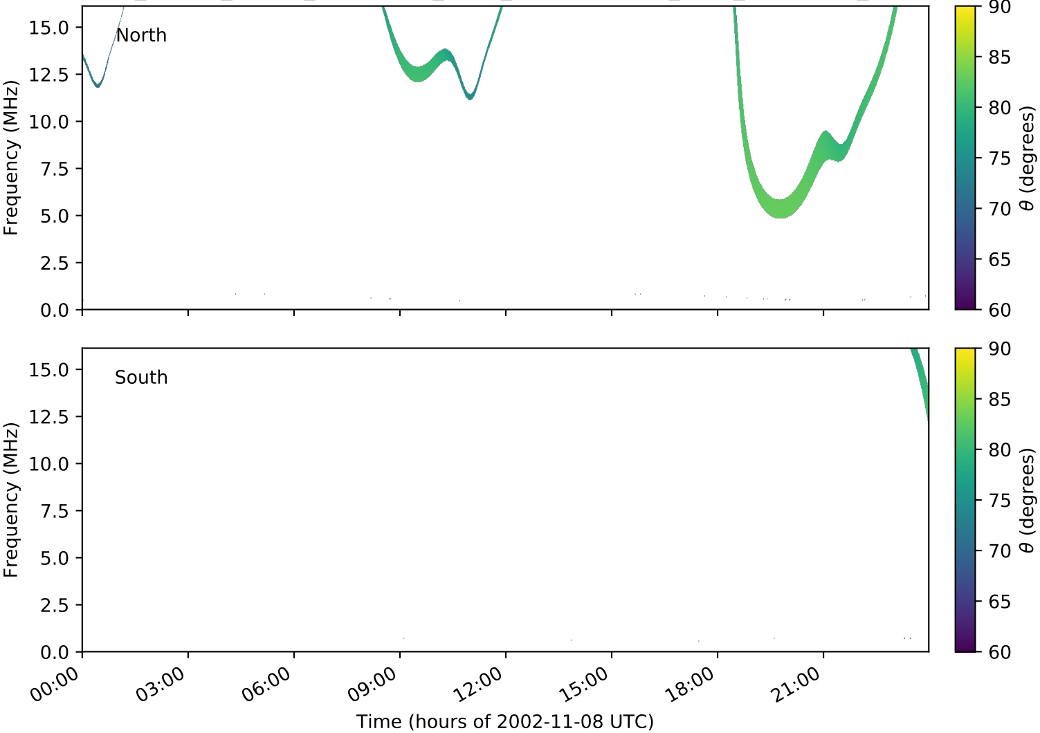
expres_cassini_jupiter_ganymede_isaac_lossc-wid1deg_3kev_20021108_v01.cdf
