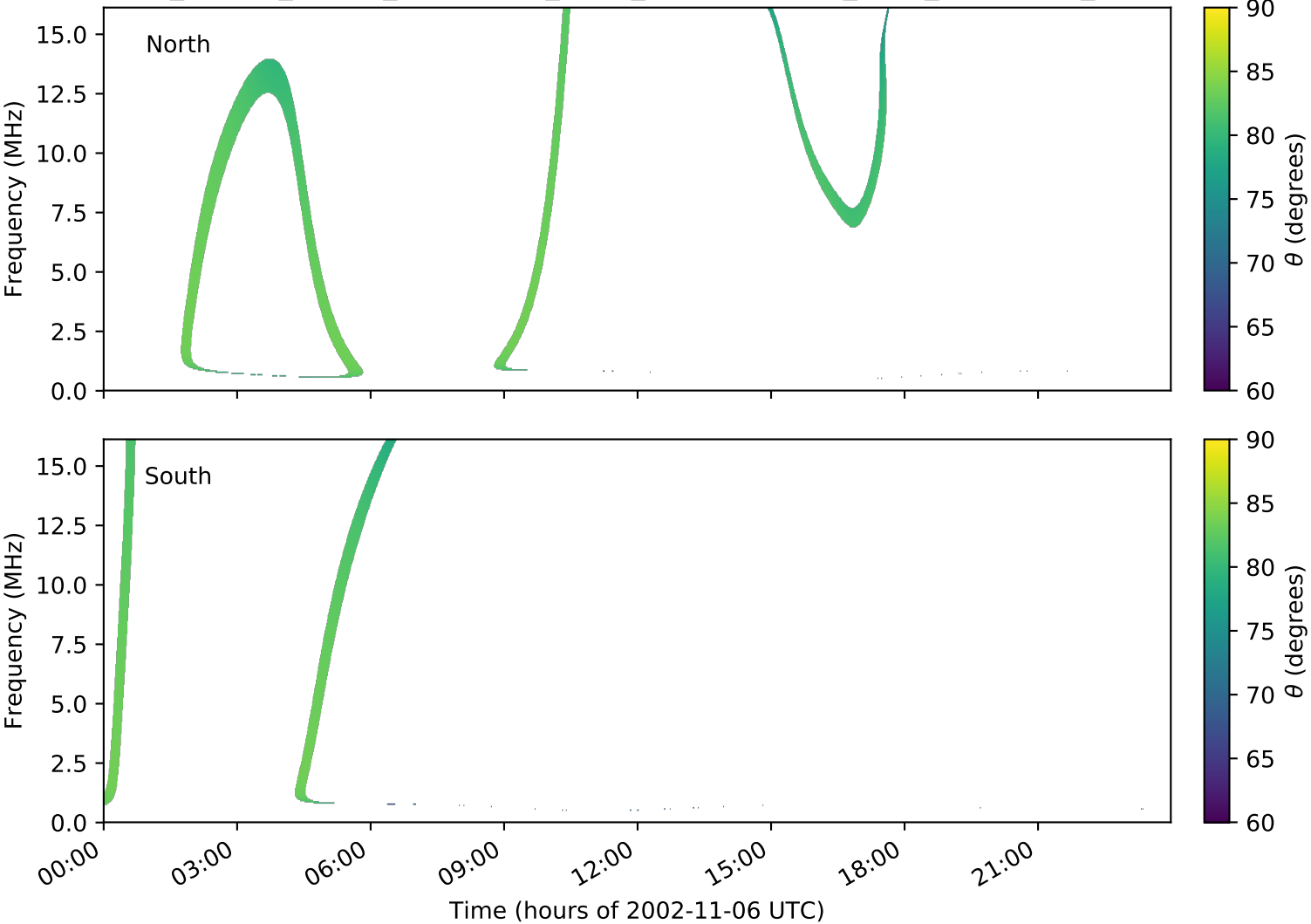
expres_cassini_jupiter_ganymede_isaac_lossc-wid1deg_3kev_20021106_v01.cdf
