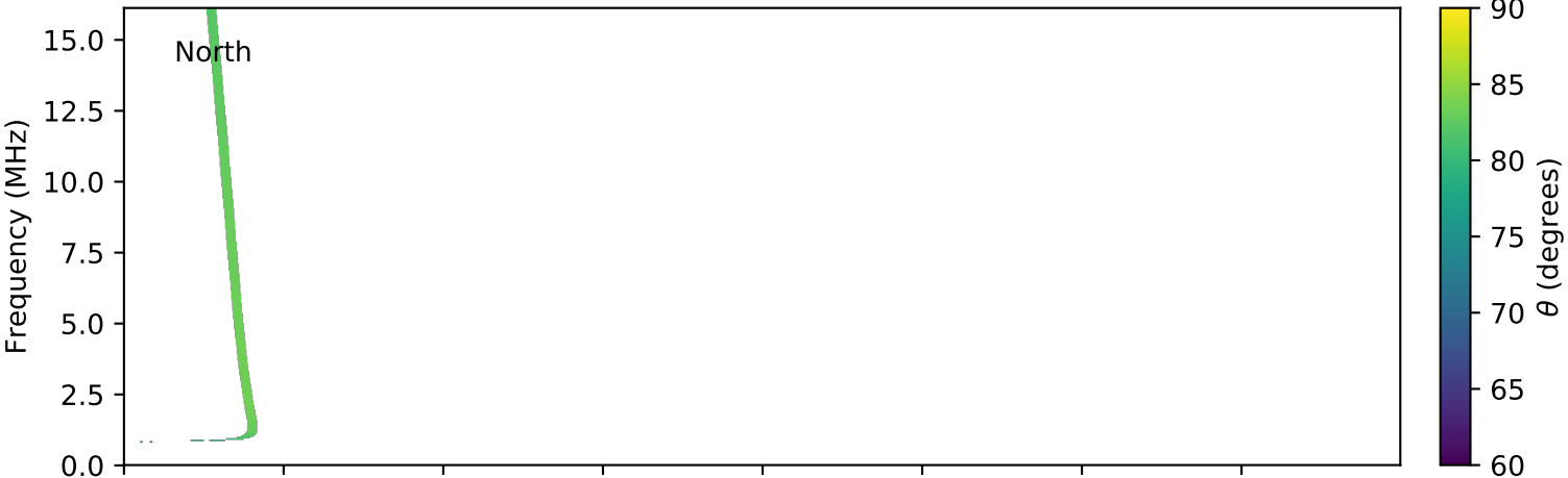
expres_cassini_jupiter_ganymede_isaac_lossc-wid1deg_3kev_20021102_v01.cdf
