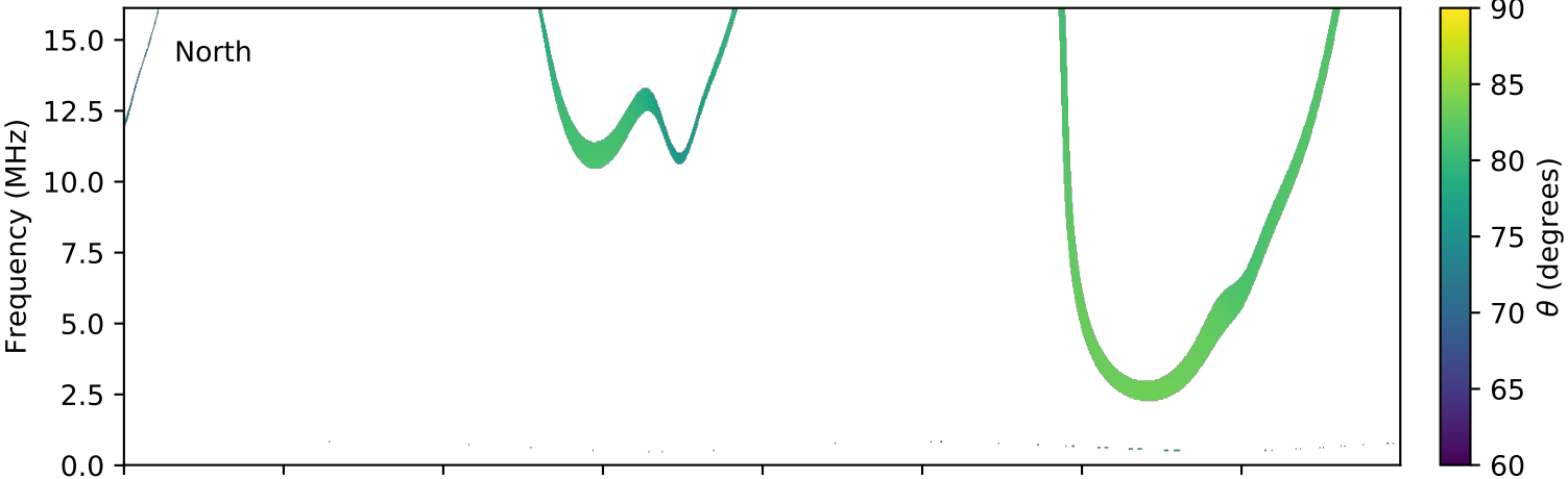
expres_cassini_jupiter_ganymede_isaac_lossc-wid1deg_3kev_20021101_v01.cdf
