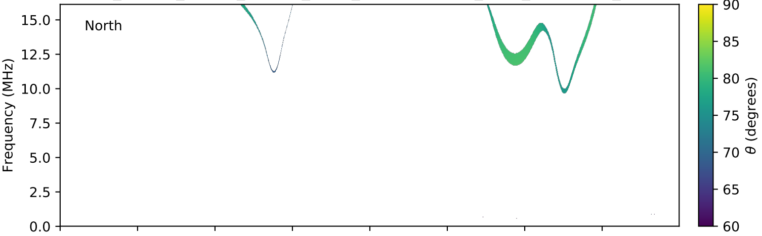
expres_cassini_jupiter_europa_isaac_lossc-wid1deg_3kev_20021130_v01.cdf
